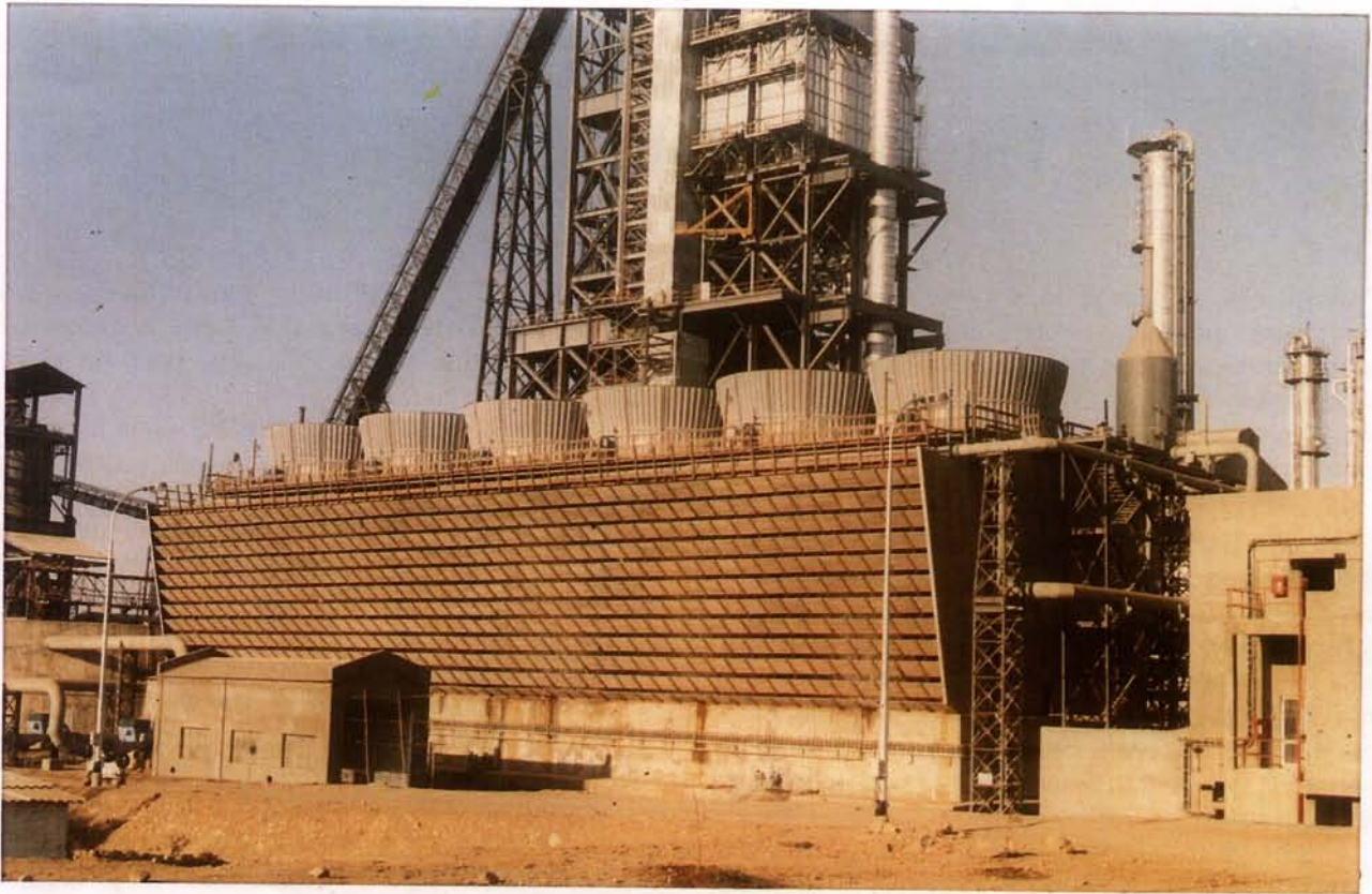
A Paharpur Class 600 Cooling Tower Model 664-4-06, Serial No. 90-2-912, at Vikram Ispat
