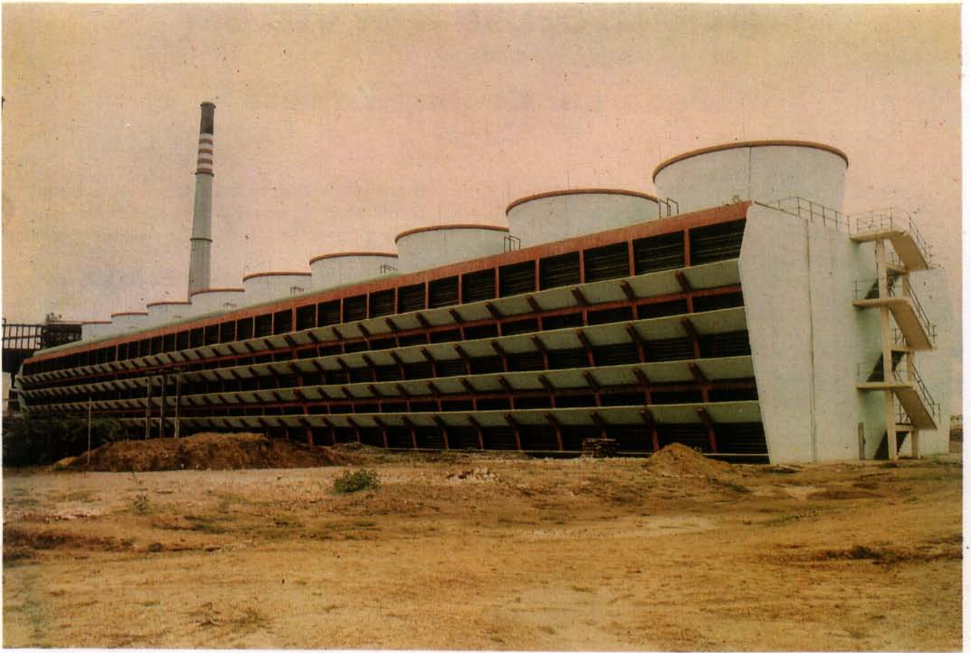
A Paharpur Class 1000 Cooling Tower Model 1513X-09. Serial No. 88-2-906 at MSEB'S Chandrapur Thermal Power Plant.
